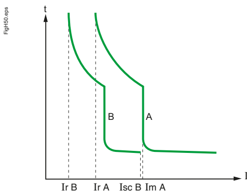
Total selectivity between CBs A and B.
