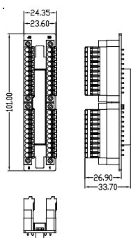
UB-10-IO32D New
