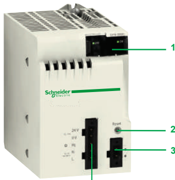
BMXCPS2000
