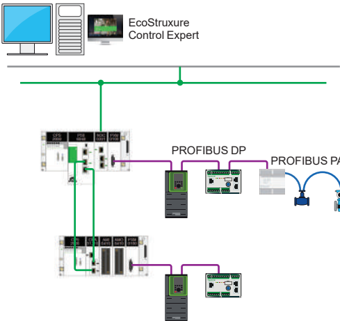
Standalone topology to connect X80 PROFIBUS DP module to M580/X80 platforms with PMEPM0100
