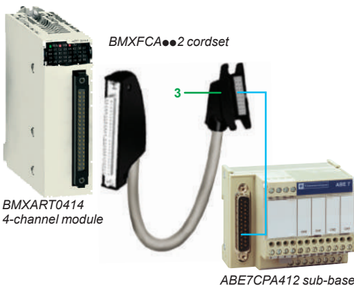
ABE7CPA412 sub-base
