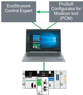
Interaction between EcoStruxure Control Expert, Prosoft Configurator for Modicon (PCM tool), and X80 PROFIBUS DP module
