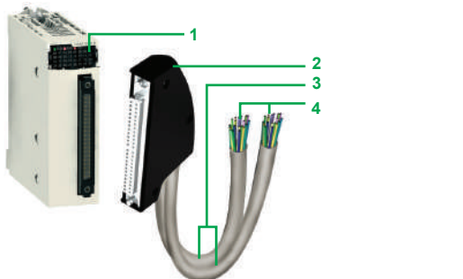
B Preassembled cordset with 40-way connector and two ends with flying leads
