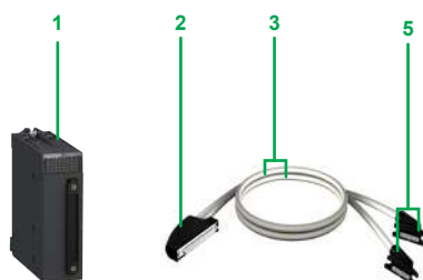
Preassembled cordset with 40-way connectors and HE10 connectors for Modicon ABE7 Telefast system
