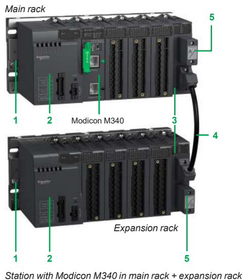
Station with Modicon M340 in main rack + expansion rack
