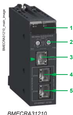
BMECRA31210
