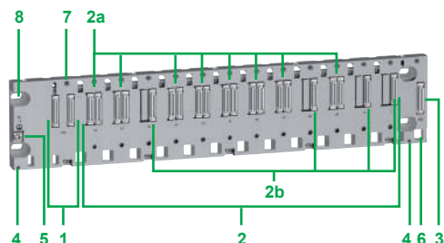
BMEXBP1200 backplane
