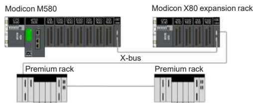
Premium X-bus expansion example
