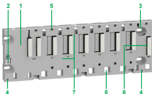
BMXXBP0600 backplane with 6 slots
