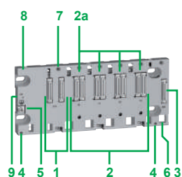
BMEXBP0400 backplane
