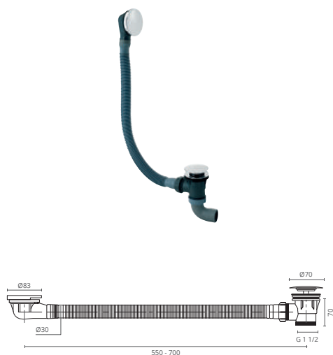
CLICK CLACK PVC
